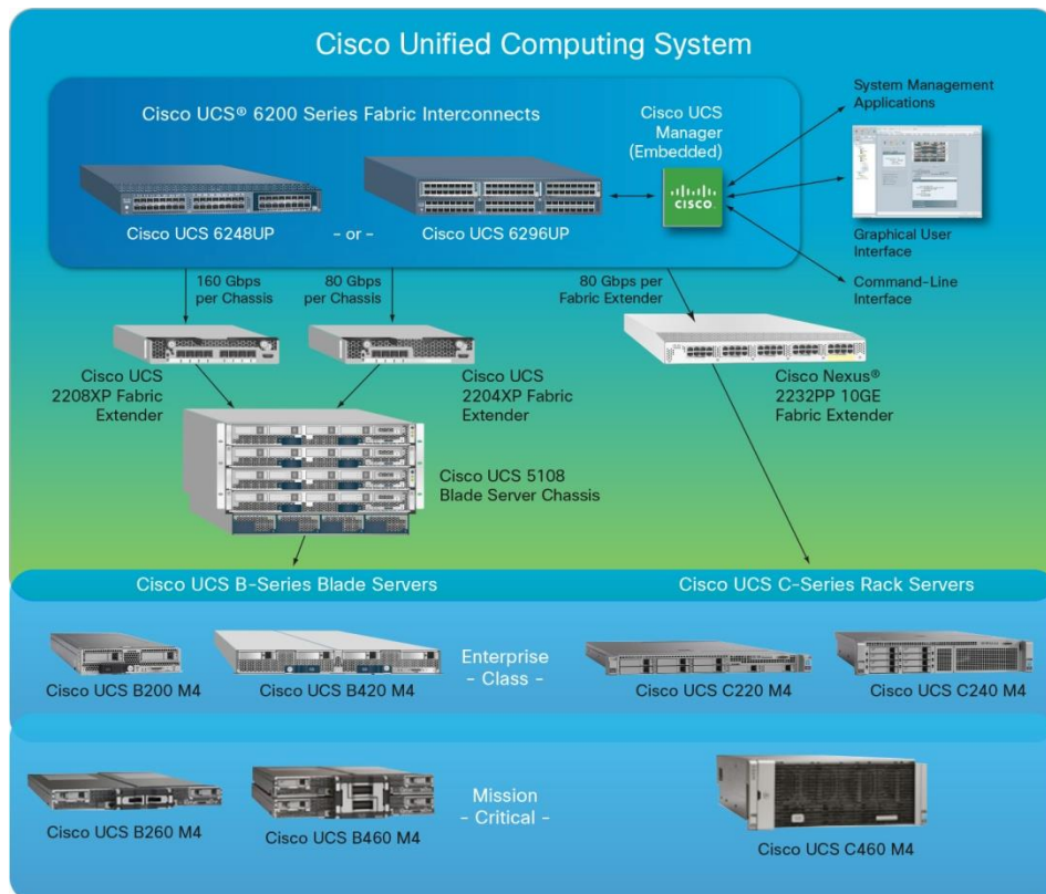
Figure 1. Cisco UCS Overview
